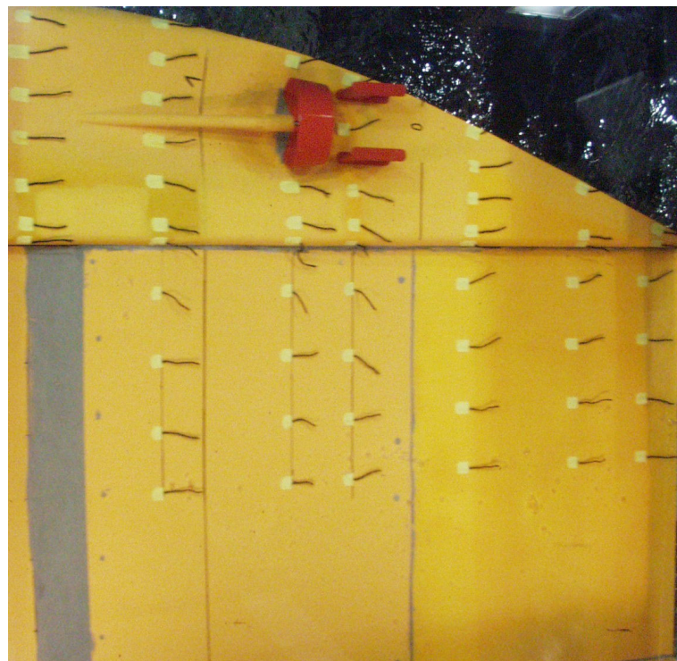
Rheinschiff, Formvariante 8, Widerstand, V = 14,0 km/h, (Vers.-Nr. 090-02-01)
